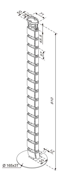
89920 screw mount type
