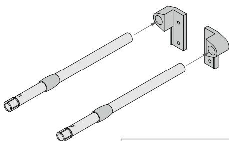
① Side rail set SRW - for wooden back
